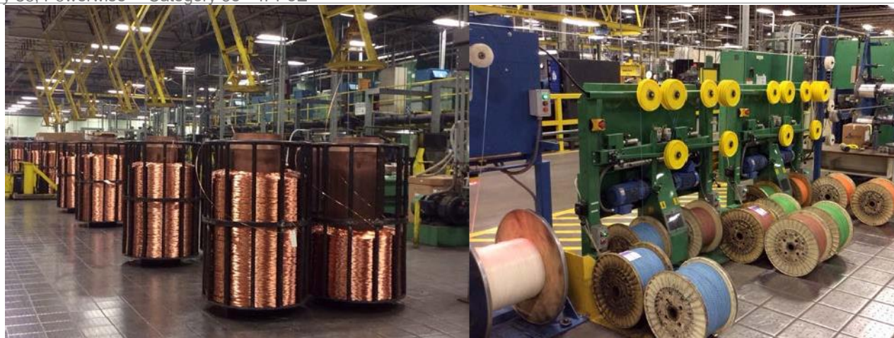
Figure 2: Photographs of Manufacturing Process
